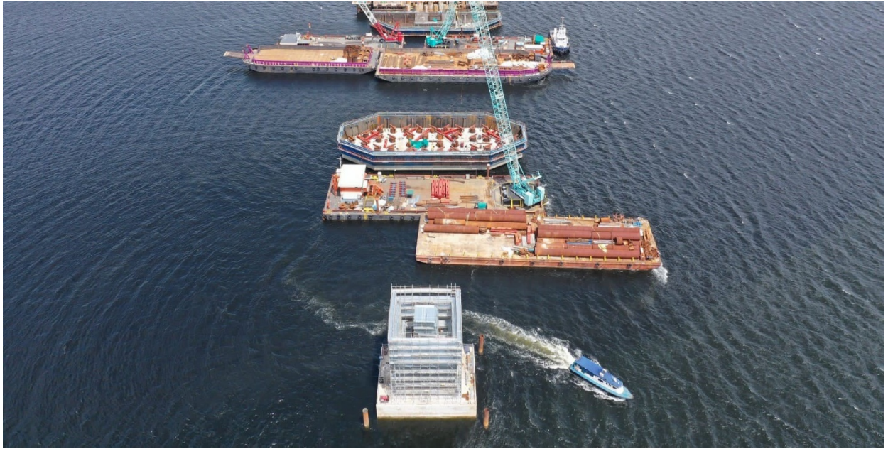
Construction of pile caps in the Straits of Johor
